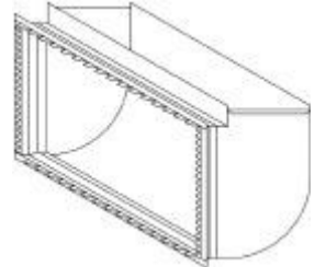
Model No. 248SF 1" Side Filter Access 1" flange out
